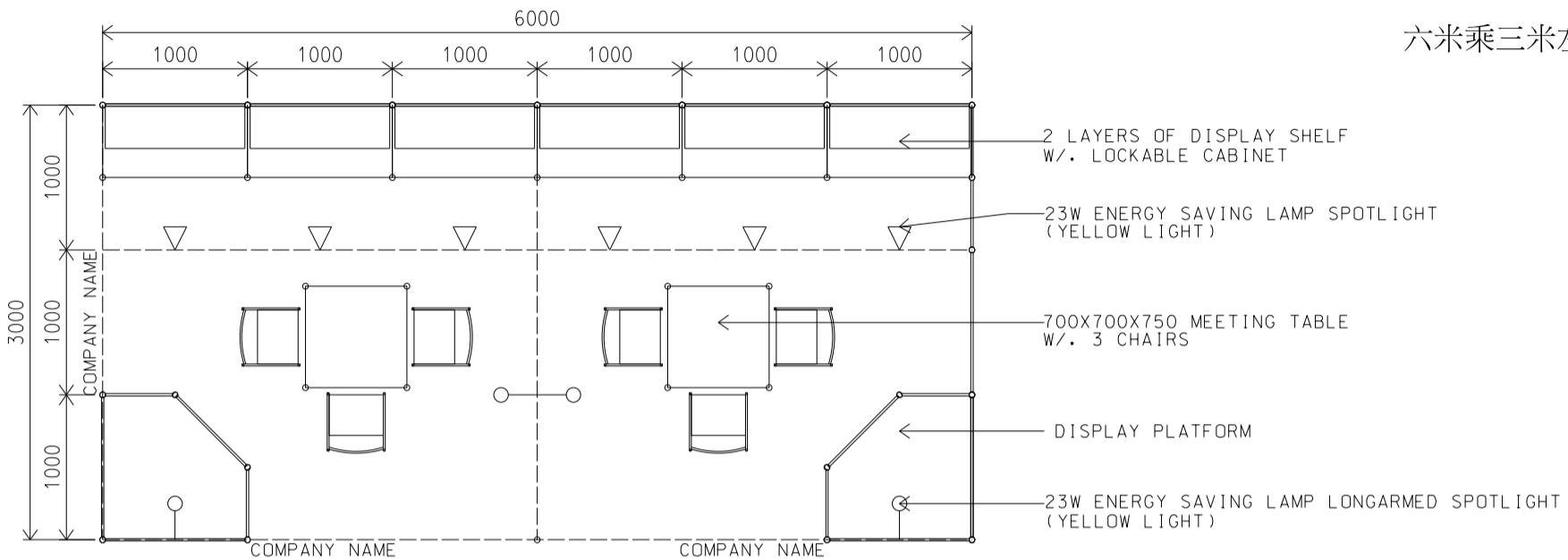
PLAN
